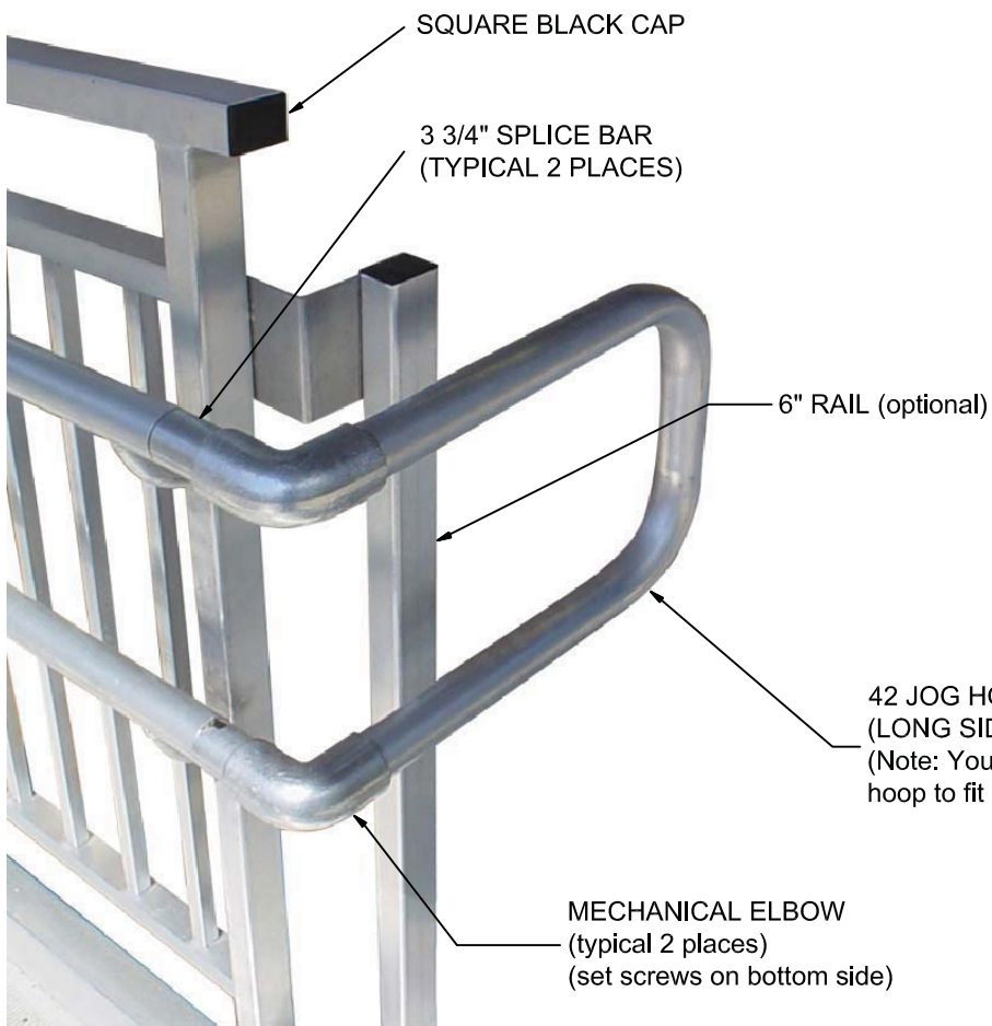
ELEVATION VIEW OF 90 DEGREE HOOP ASSEMBLY
