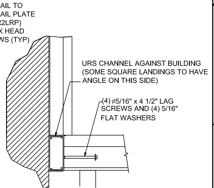
SECTION VIEW OF LANDING TO BUILDING
