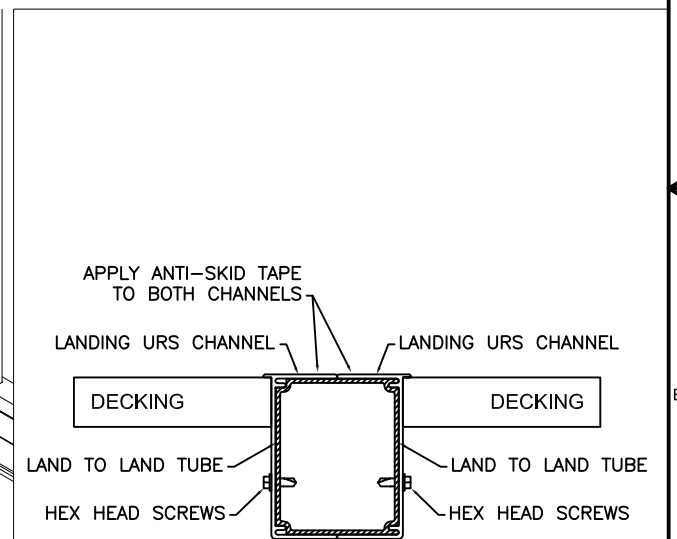
SECTION VIEW OF LAND TO LAND CONNECTOR
