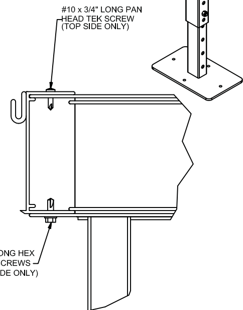
SECTION VIEW OF LANDING
